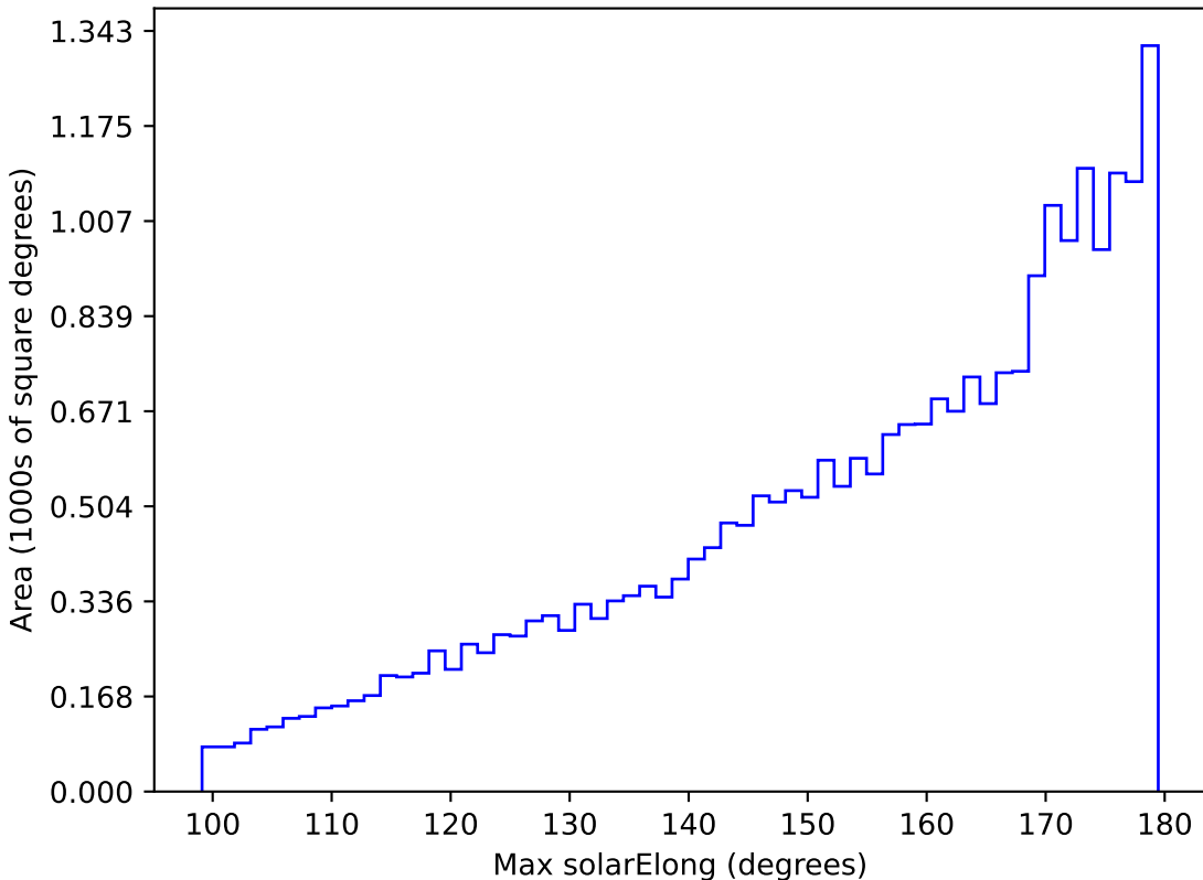
too_ignore_5_4v3.4_10yrs All sky r band: Max solarElong
