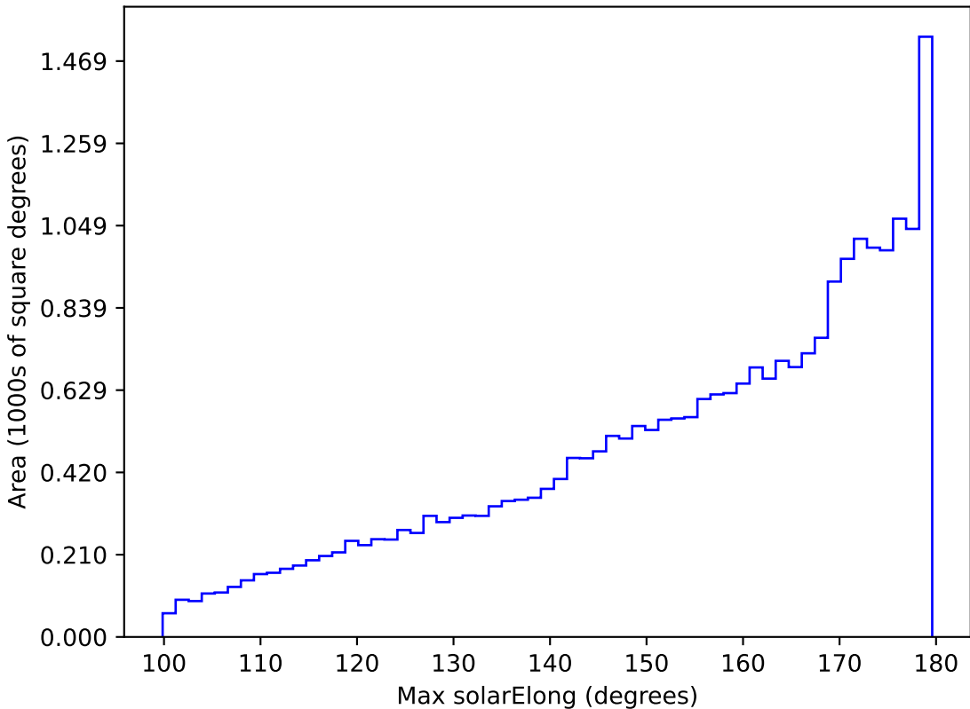
too_ignore_5_4v3.4_10yrs All sky all bands: Max solarElong
