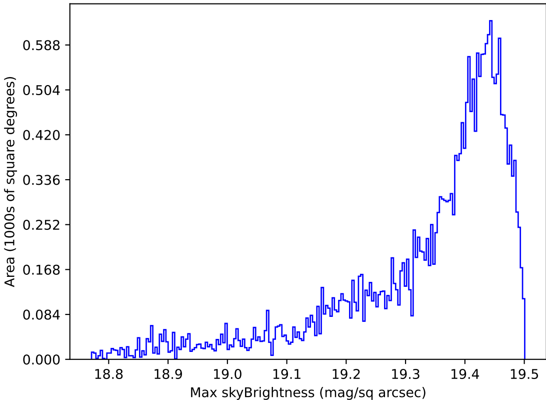
too_ignore_5_4v3.4_10yrs Yr 1 z band: Max skyBrightness
