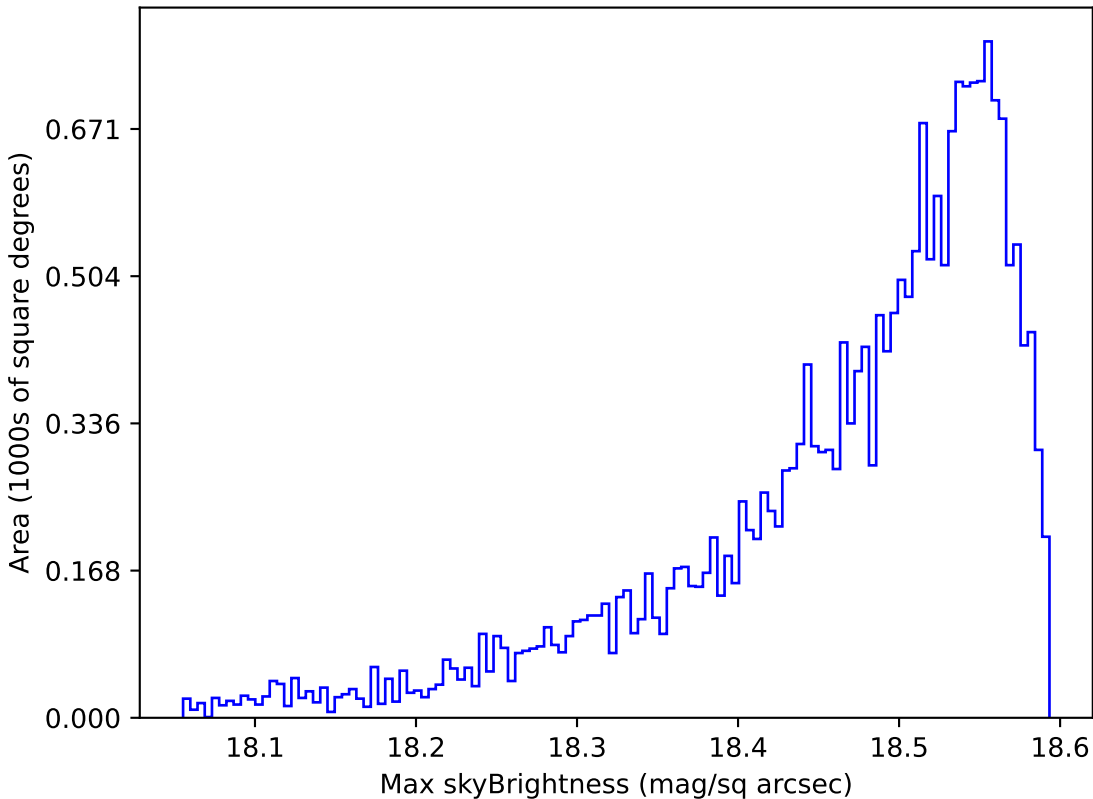
too_ignore_5_4v3.4_10yrs Yr 1 y band: Max skyBrightness
