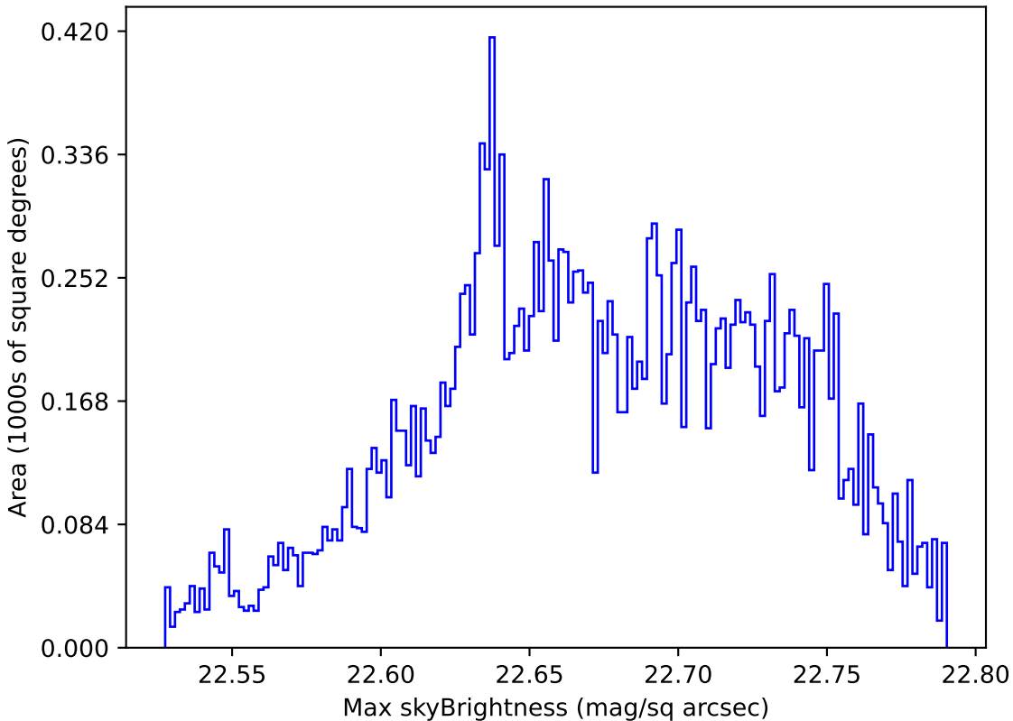
too_ignore_5_4v3.4_10yrs Yr 1 u band: Max skyBrightness
