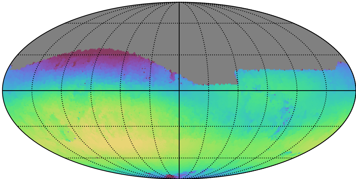
too_ignore_5_4v3.4_10yrs Yr 1 r band: Max skyBrightness
