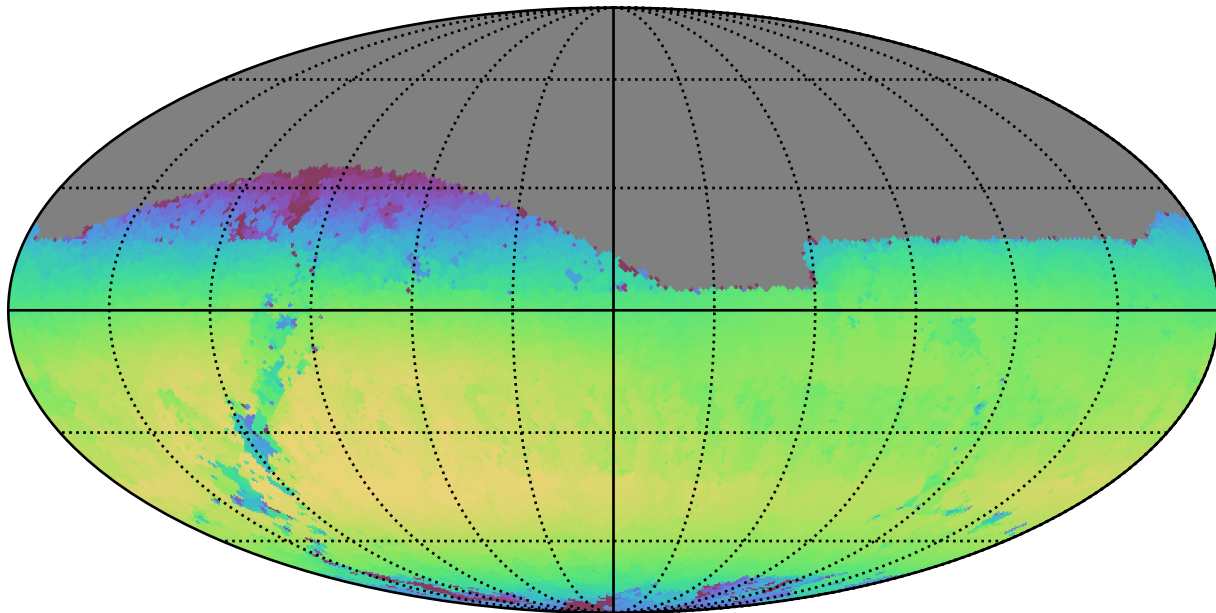
too_ignore_5_4v3.4_10yrs Yr 1 i band: Max skyBrightness
