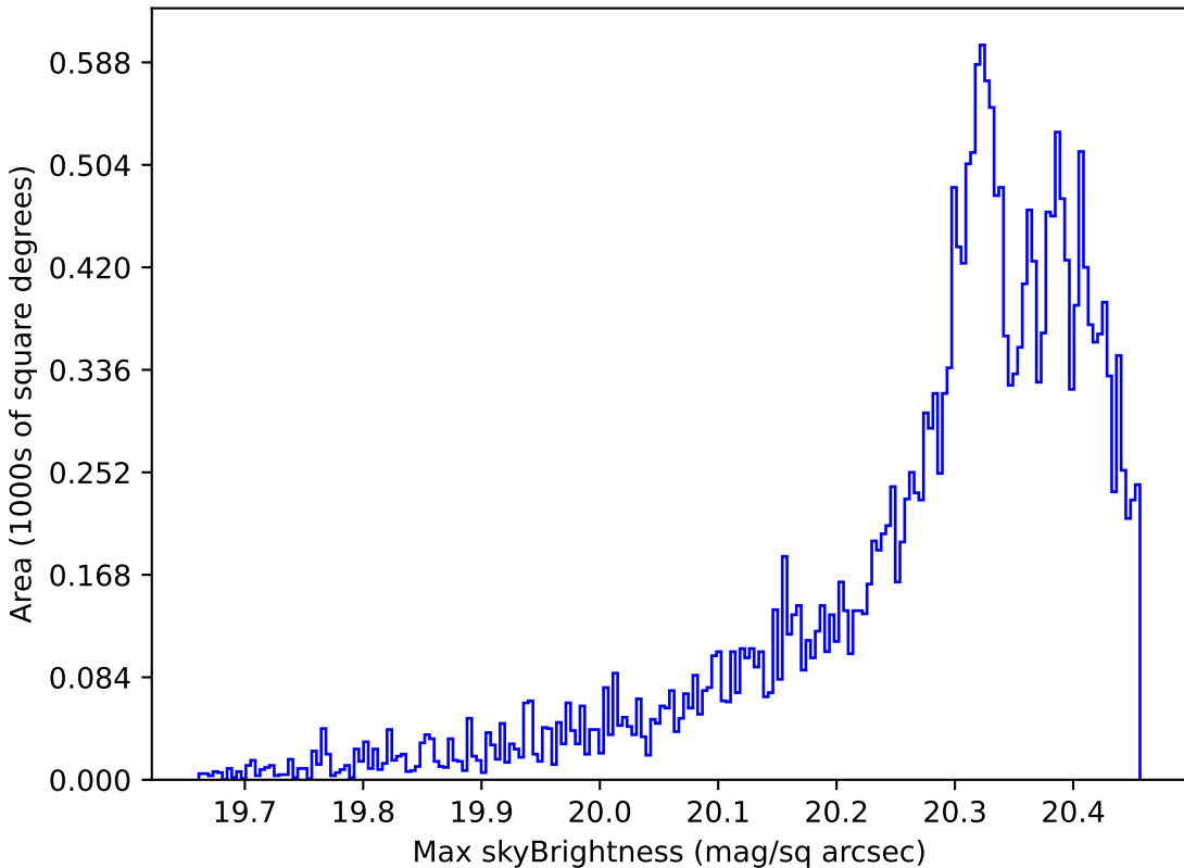
too_ignore_5_4v3.4_10yrs Yr 1 i band: Max skyBrightness
