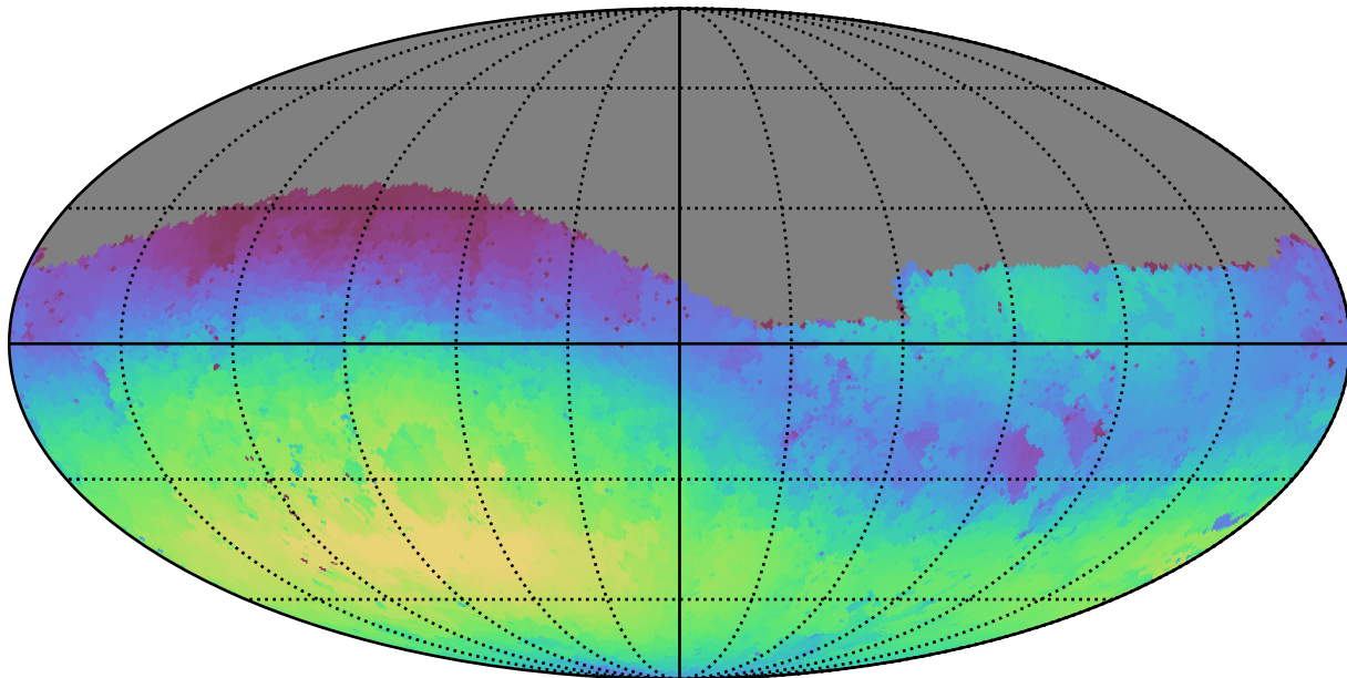
too_ignore_5_4v3.4_10yrs Yr 1 g band: Max skyBrightness
