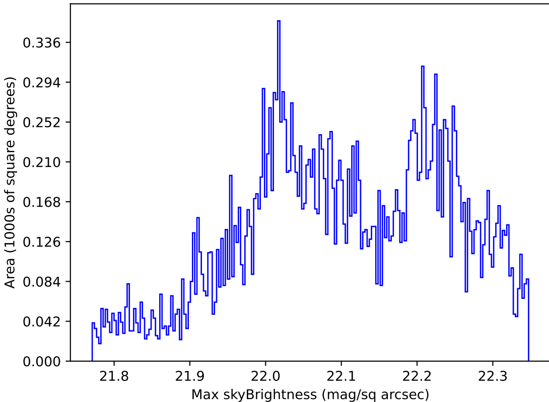
too_ignore_5_4v3.4_10yrs Yr 1 g band: Max skyBrightness
