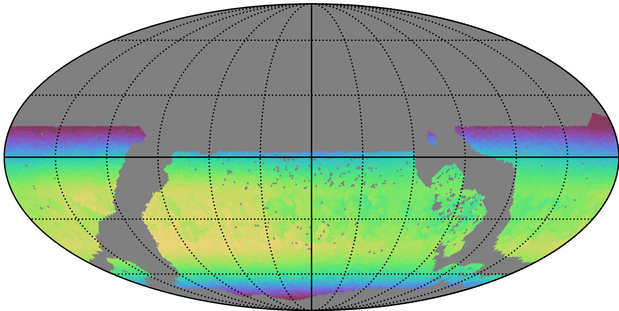
too_ignore_5_4v3.4_10yrs WFD z band: Max skyBrightness
