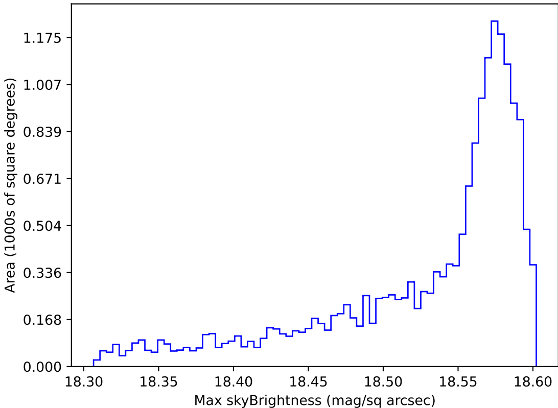
too_ignore_5_4v3.4_10yrs WFD y band: Max skyBrightness
