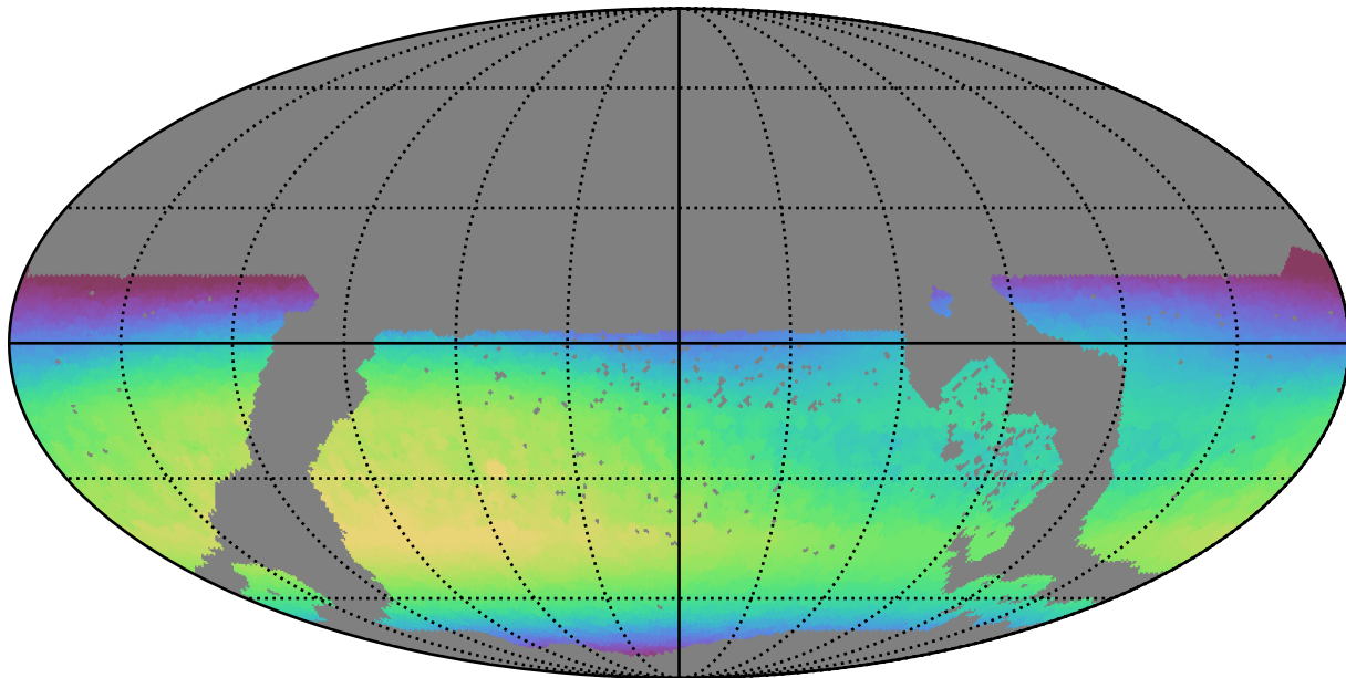
too_ignore_5_4v3.4_10yrs WFD i band: Max skyBrightness
