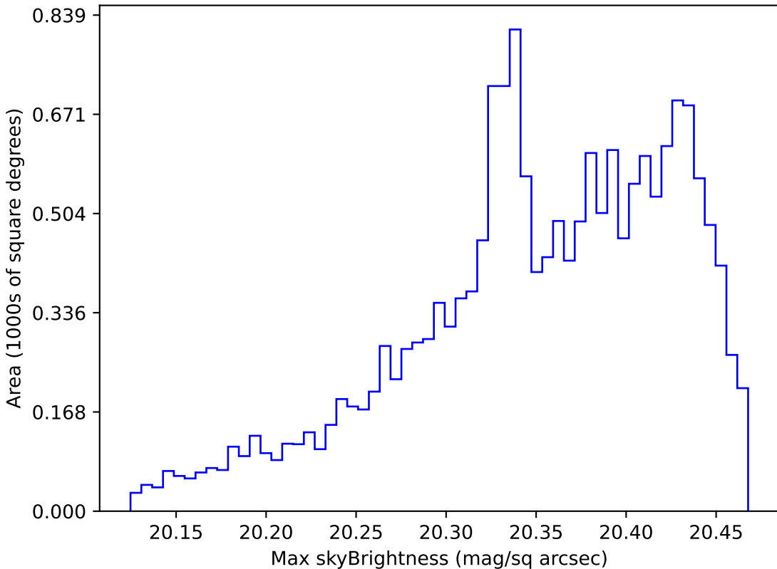
too_ignore_5_4v3.4_10yrs WFD i band: Max skyBrightness
