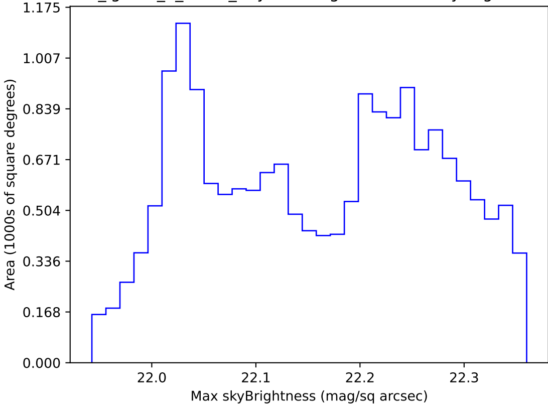
too_ignore_5_4v3.4_10yrs WFD g band: Max skyBrightness
