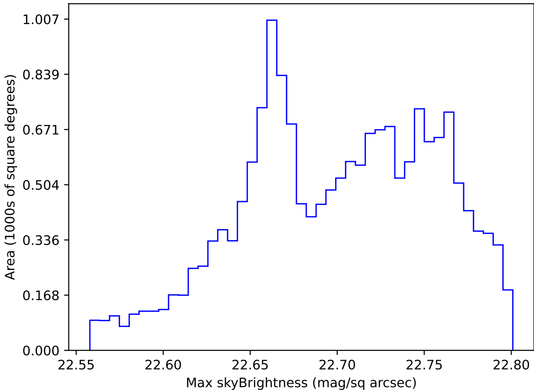
too_ignore_5_4v3.4_10yrs WFD all bands: Max skyBrightness
