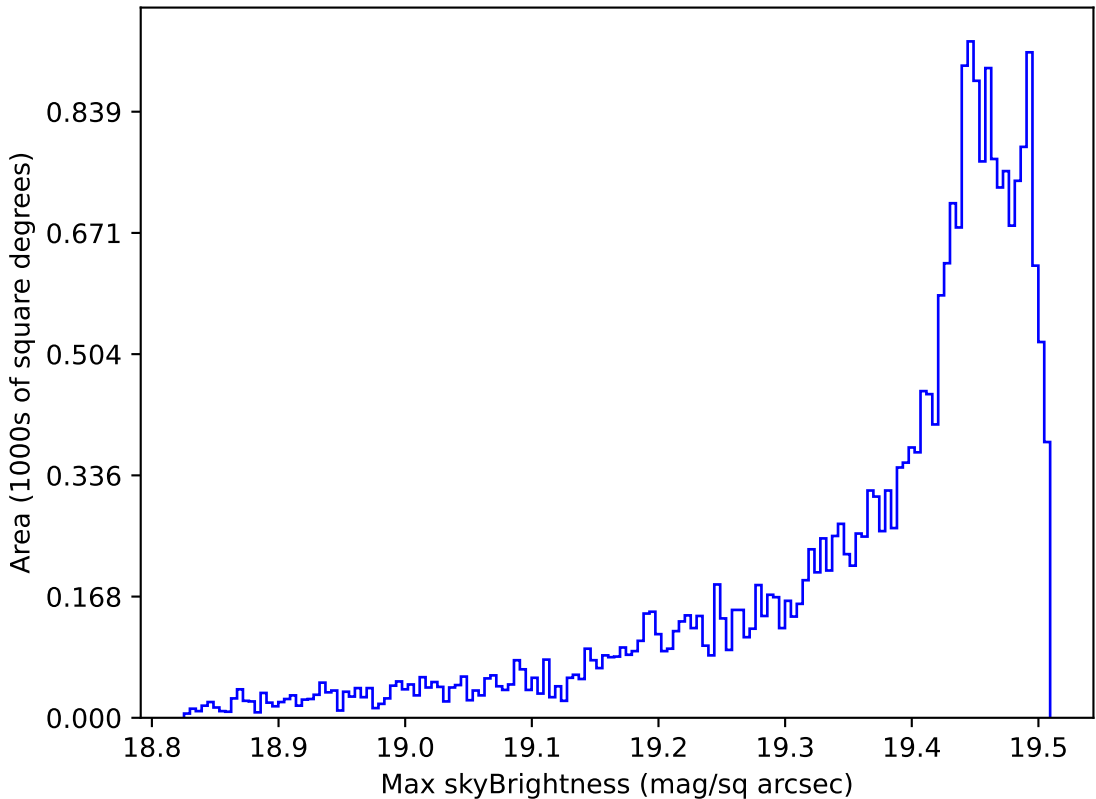
too_ignore_5_4v3.4_10yrs All sky z band: Max skyBrightness
