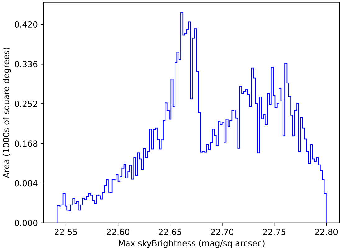
too_ignore_5_4v3.4_10yrs All sky u band: Max skyBrightness
