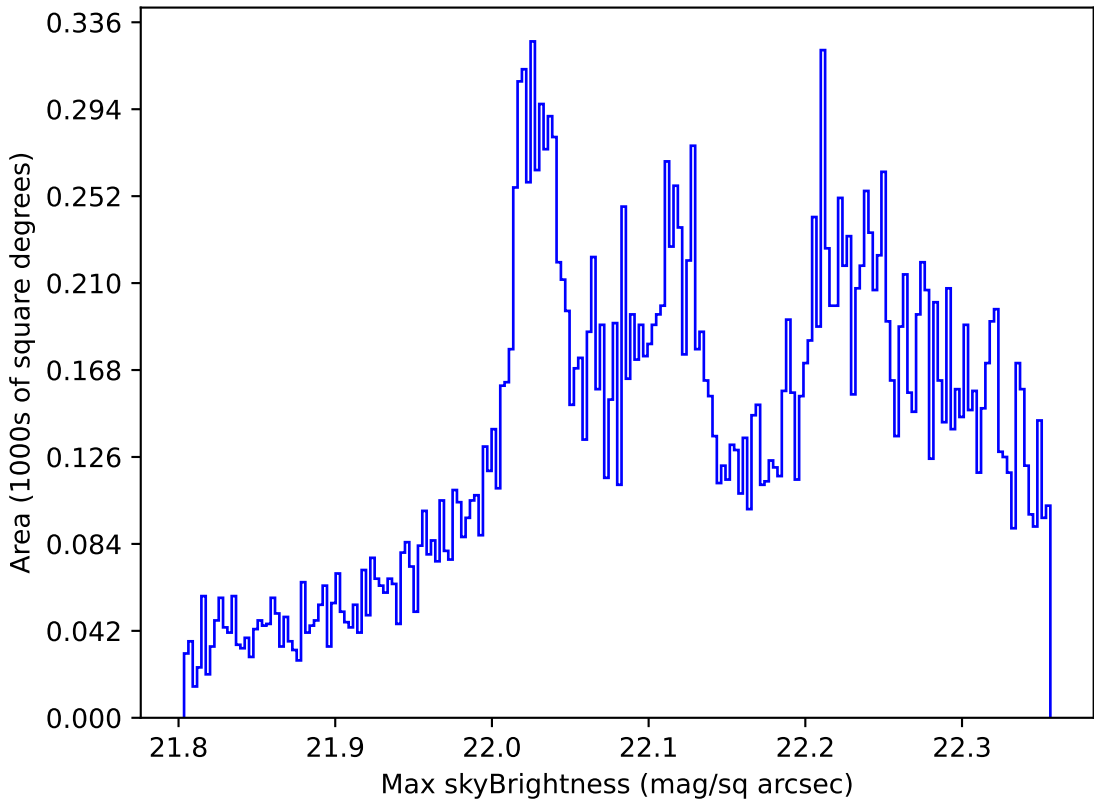
too_ignore_5_4v3.4_10yrs All sky g band: Max skyBrightness
