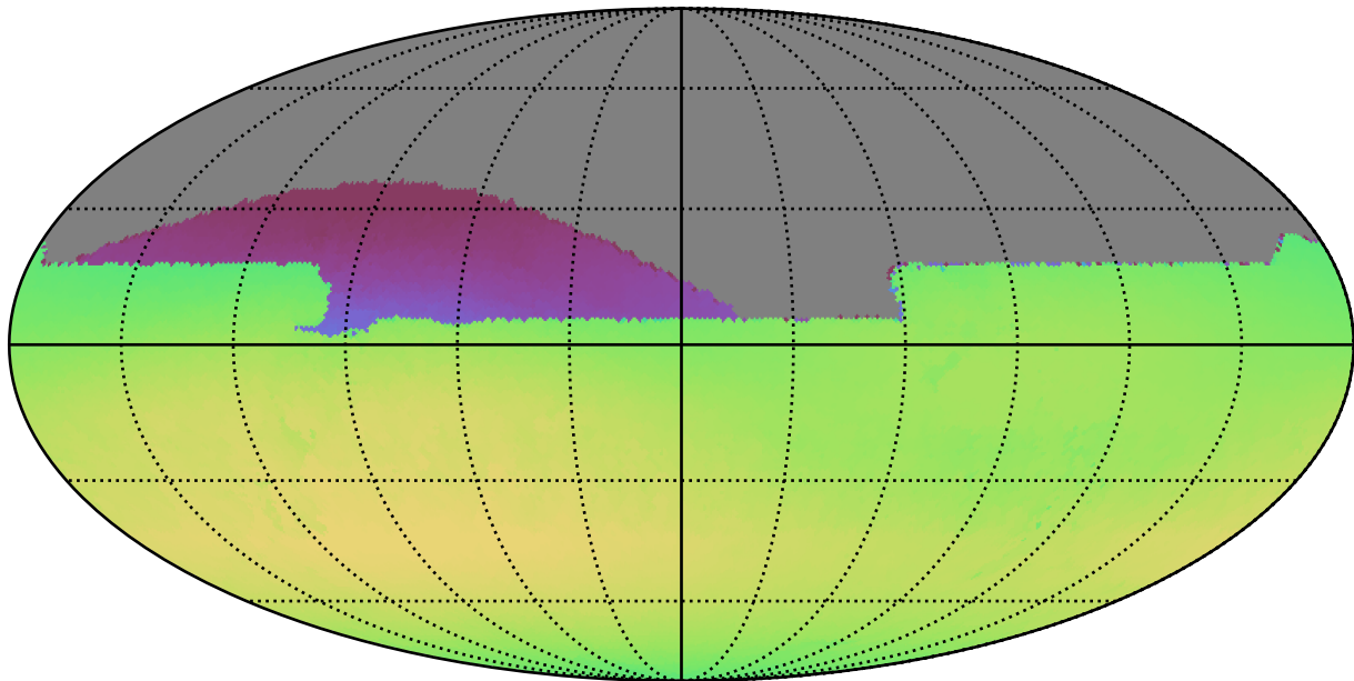
too_ignore_5_4v3.4_10yrs All sky all bands: Max skyBrightness
