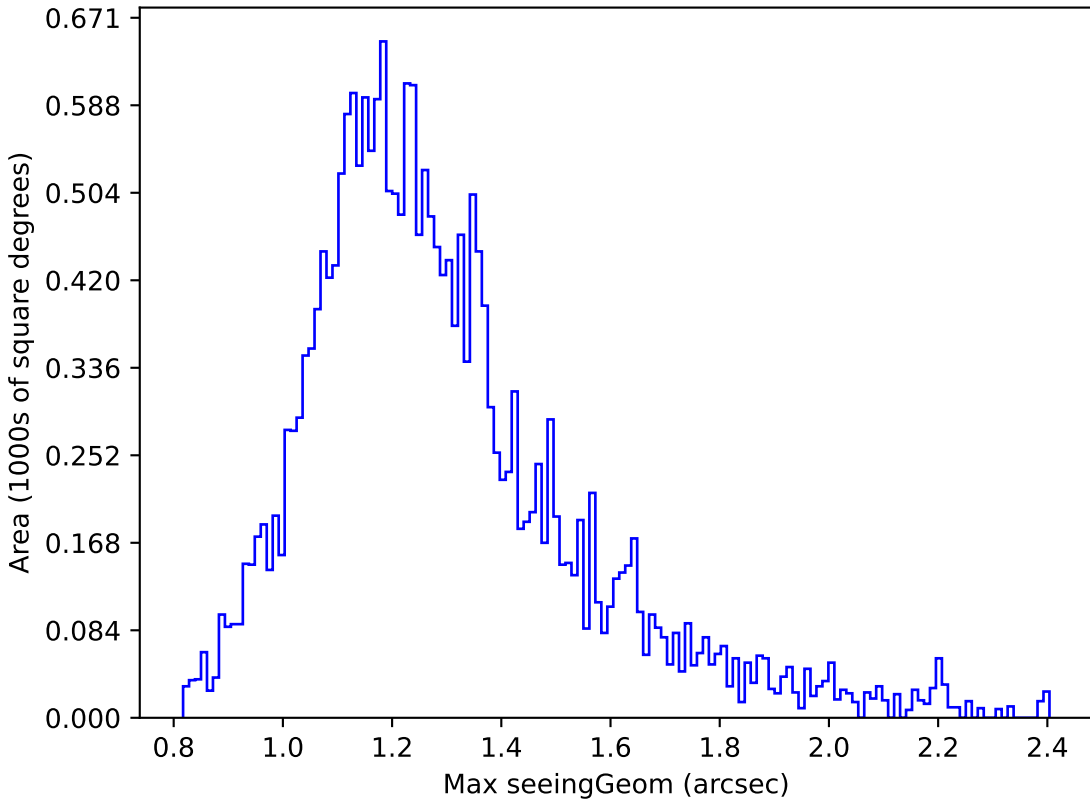
too_ignore_5_4v3.4_10yrs Yr 1 y band: Max seeingGeom
