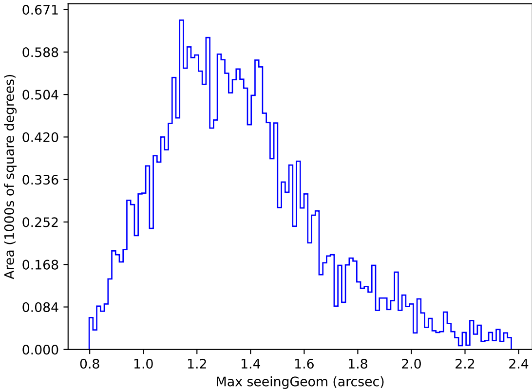
too_ignore_5_4v3.4_10yrs Yr 1 r band: Max seeingGeom
