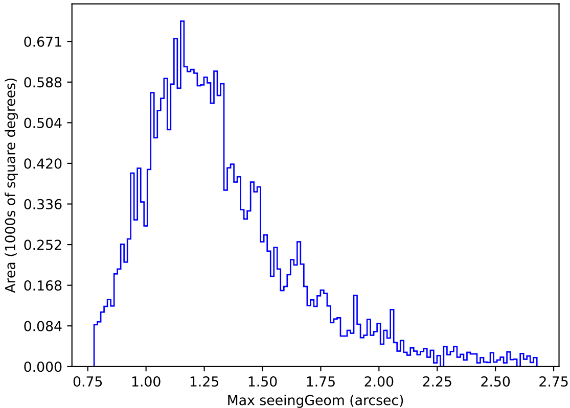
too_ignore_5_4v3.4_10yrs Yr 1 g band: Max seeingGeom
