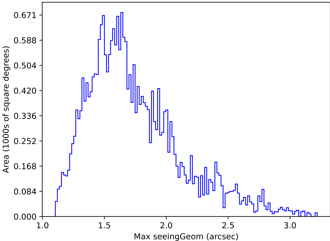
too_ignore_5_4v3.4_10yrs Yr 1 all bands: Max seeingGeom
