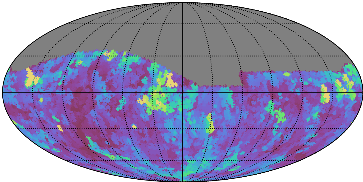
too_ignore_5_4v3.4_10yrs Yr 1 z band: Max seeingEff
