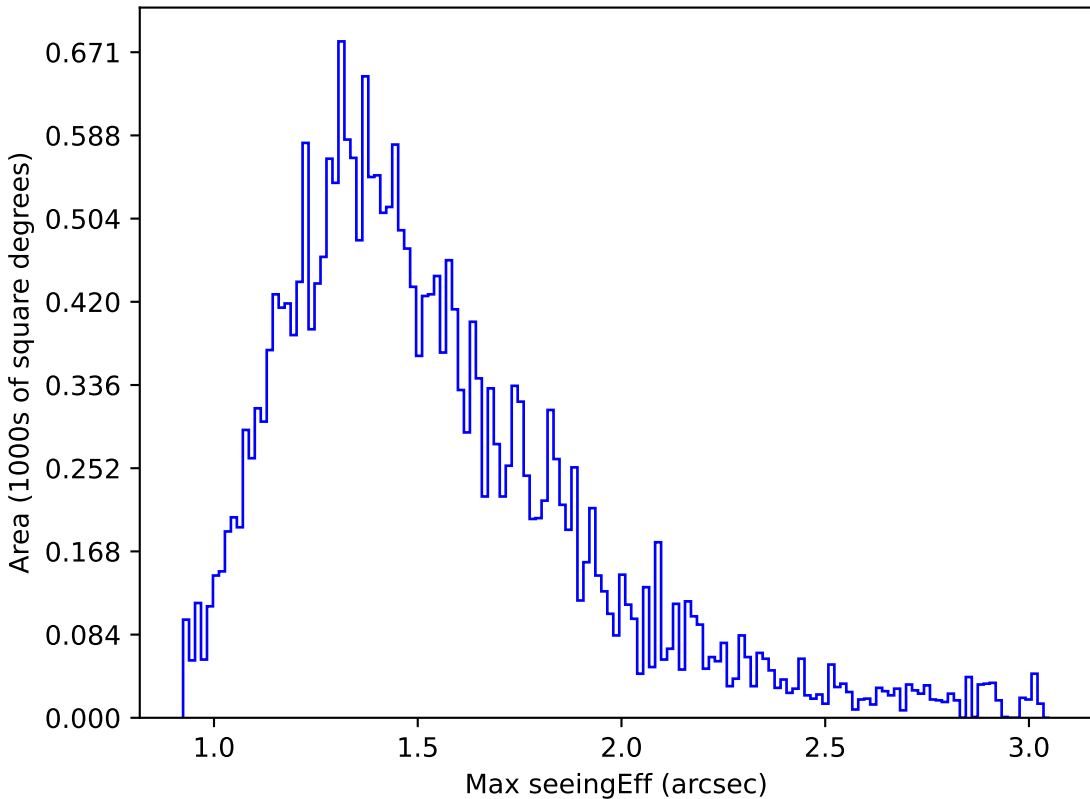
too_ignore_5_4v3.4_10yrs Yr 1 z band: Max seeingEff
