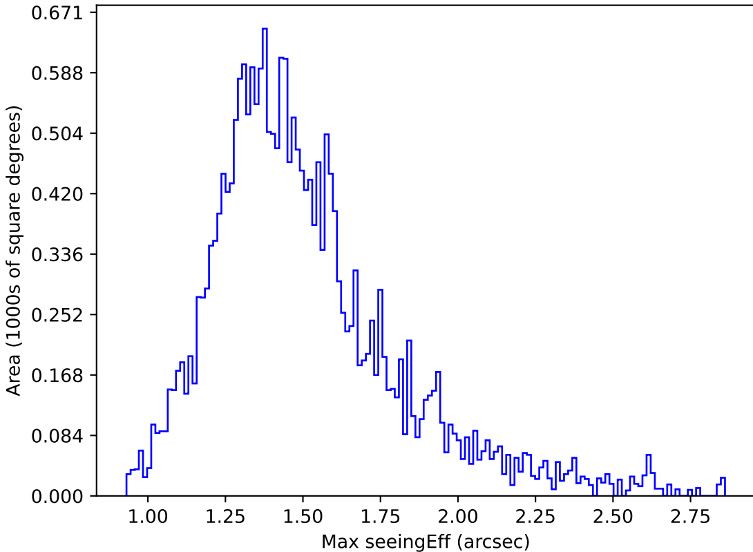
too_ignore_5_4v3.4_10yrs Yr 1 y band: Max seeingEff
