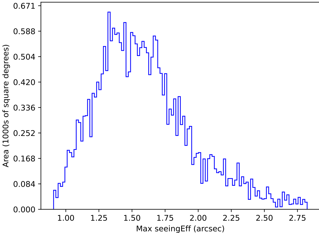
too_ignore_5_4v3.4_10yrs Yr 1 r band: Max seeingEff
