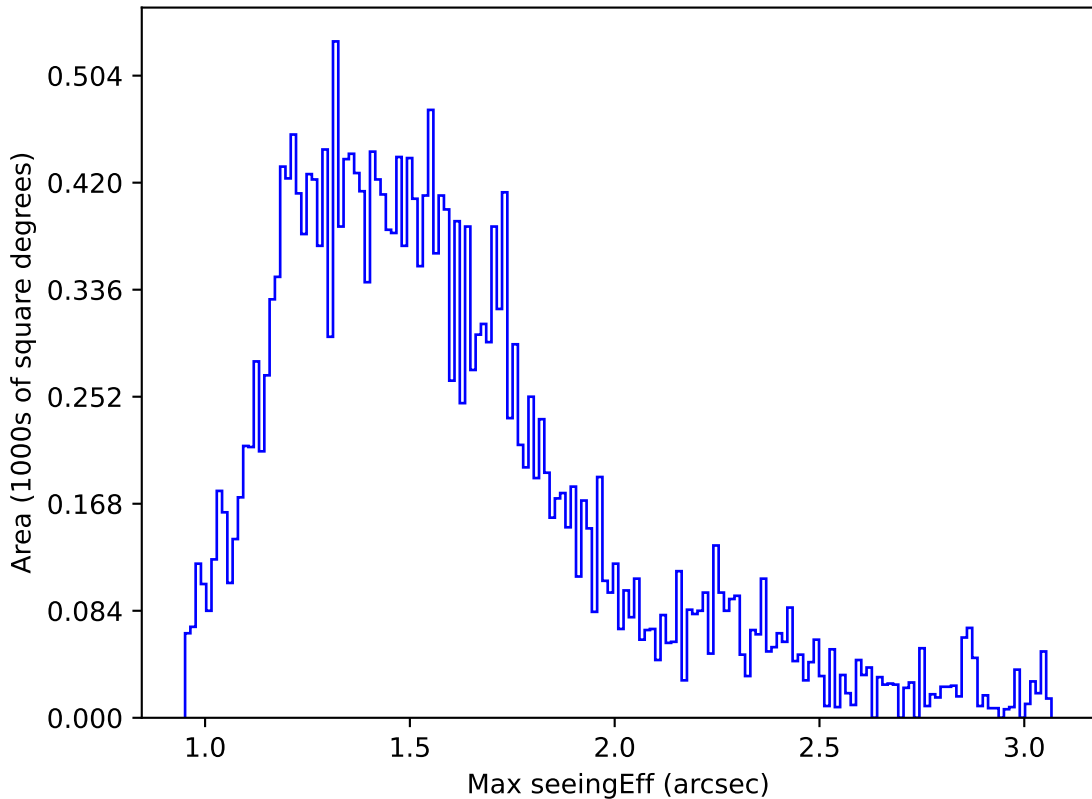
too_ignore_5_4v3.4_10yrs Yr 1 i band: Max seeingEff
