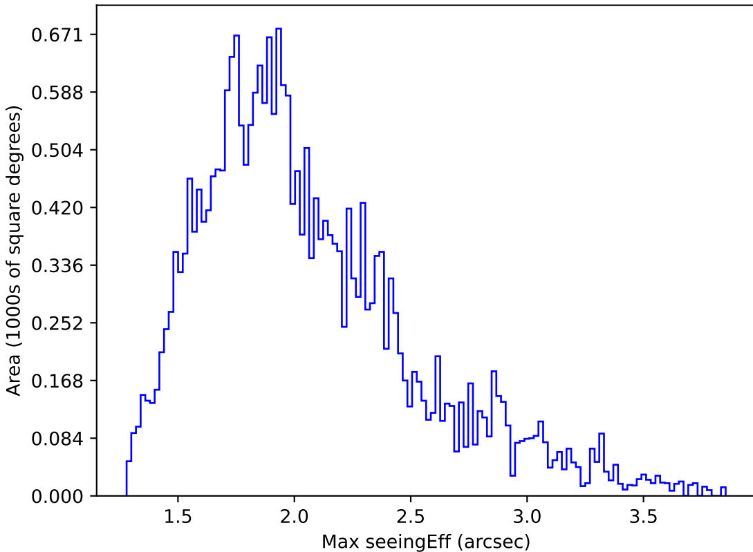
too_ignore_5_4v3.4_10yrs Yr 1 all bands: Max seeingEff
