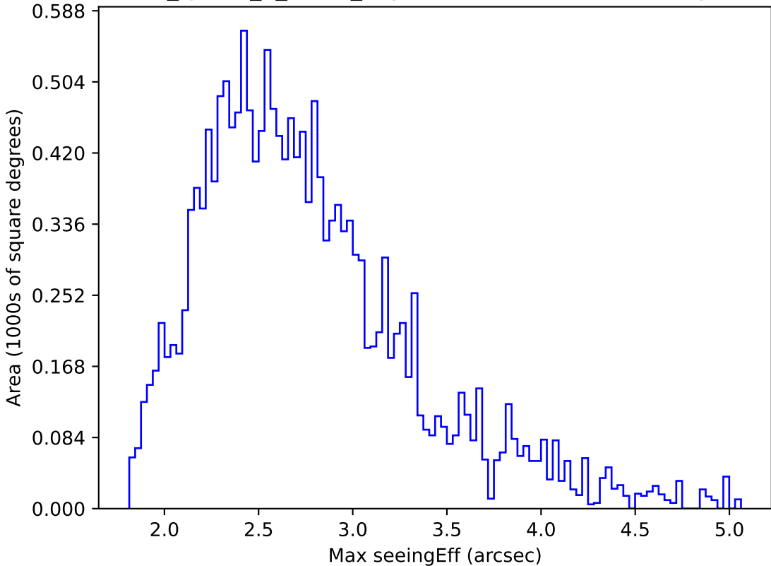
too_ignore_5_4v3.4_10yrs WFD r band: Max seeingEff
