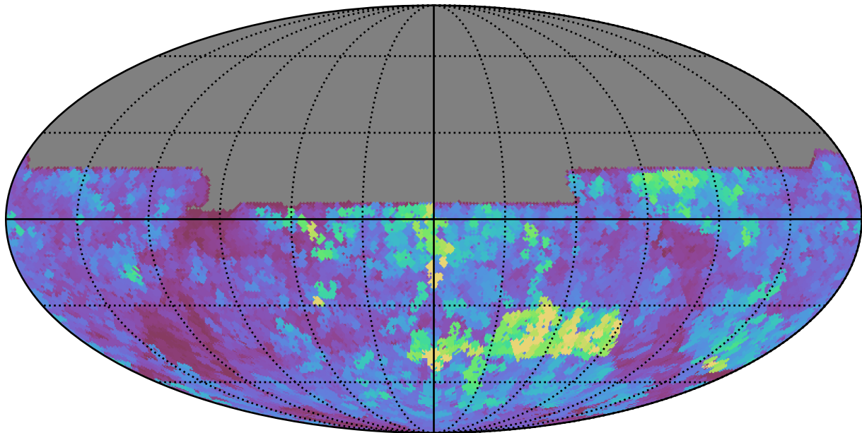
too_ignore_5_4v3.4_10yrs All sky y band: Max seeingEff
