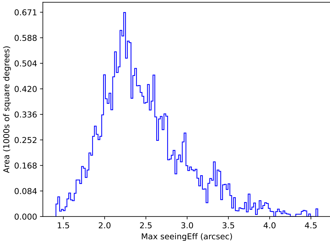
too_ignore_5_4v3.4_10yrs All sky u band: Max seeingEff
