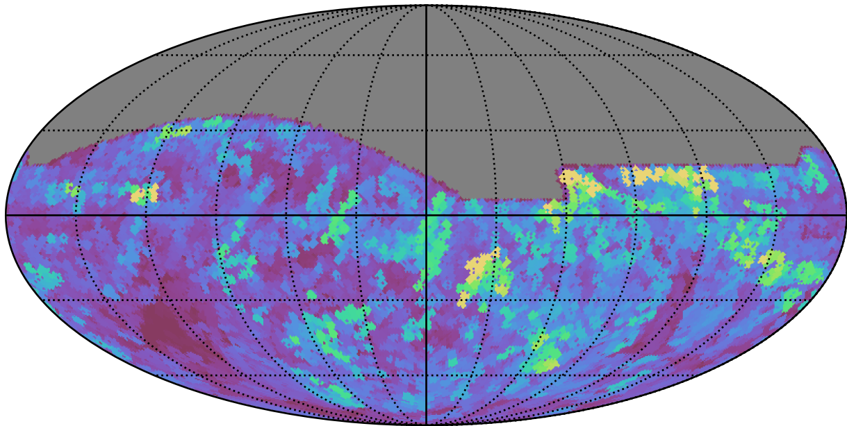
too_ignore_5_4v3.4_10yrs All sky r band: Max seeingEff
