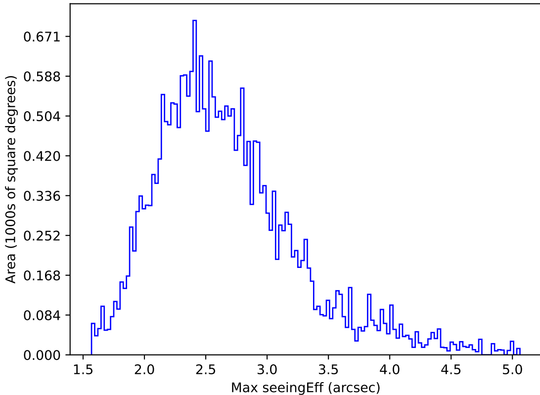
too_ignore_5_4v3.4_10yrs All sky r band: Max seeingEff
