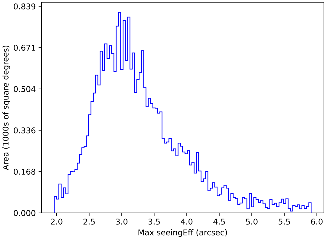
too_ignore_5_4v3.4_10yrs All sky all bands: Max seeingEff
