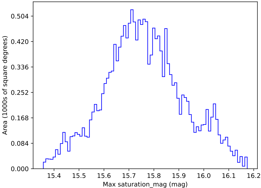
too_ignore_5_4v3.4_10yrs WFD r band: Max saturation_mag
