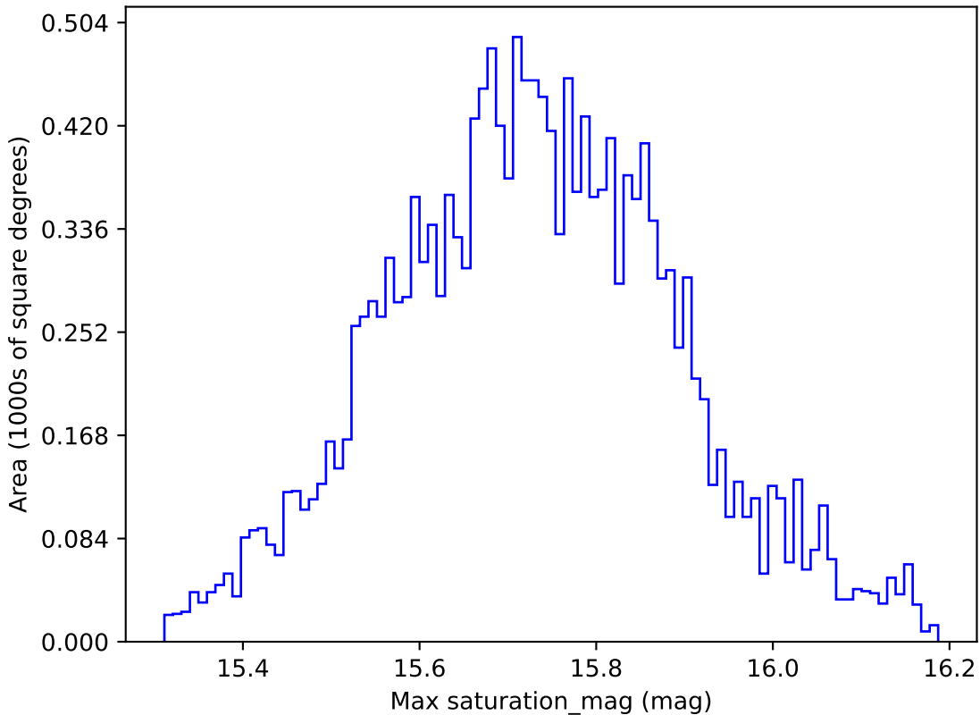
too_ignore_5_4v3.4_10yrs WFD g band: Max saturation_mag
