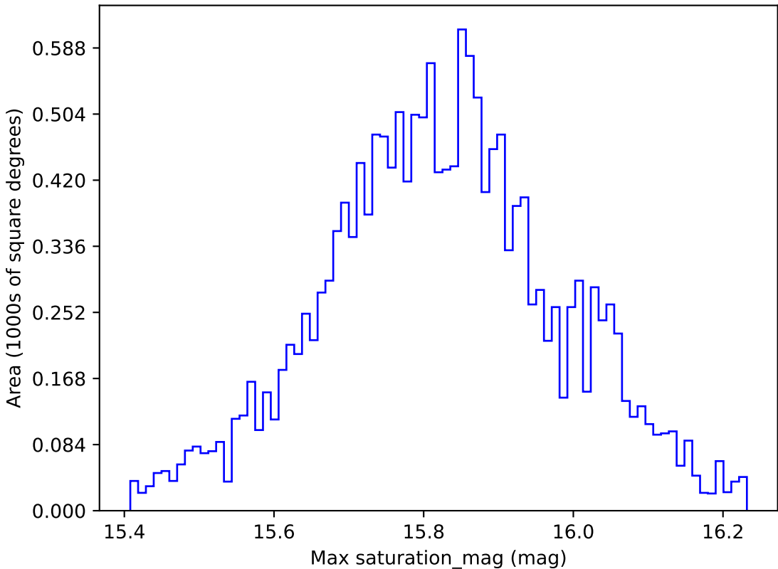
too_ignore_5_4v3.4_10yrs WFD all bands: Max saturation_mag
