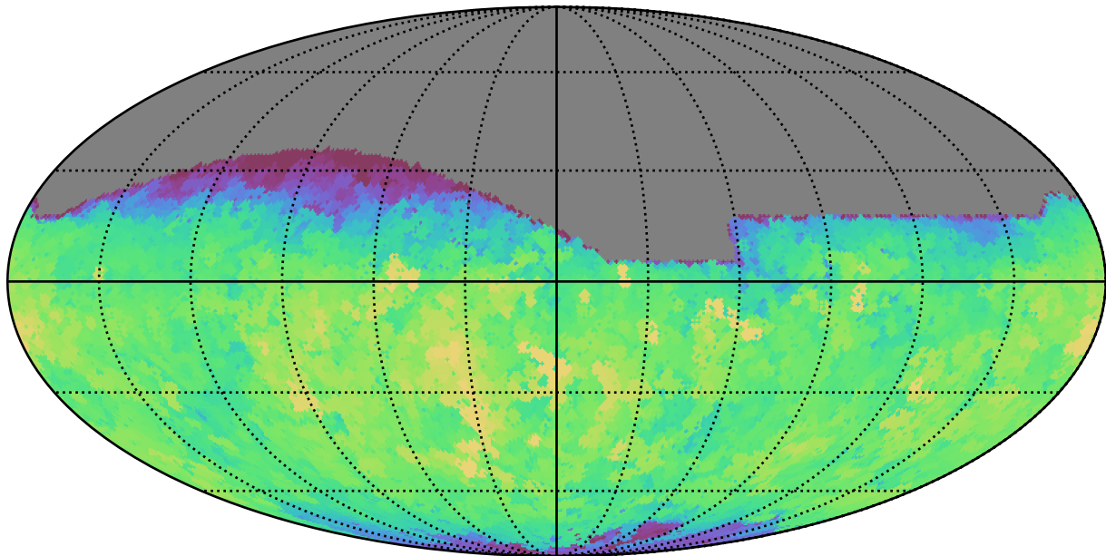
too_ignore_5_4v3.4_10yrs All sky g band: Max saturation_mag
