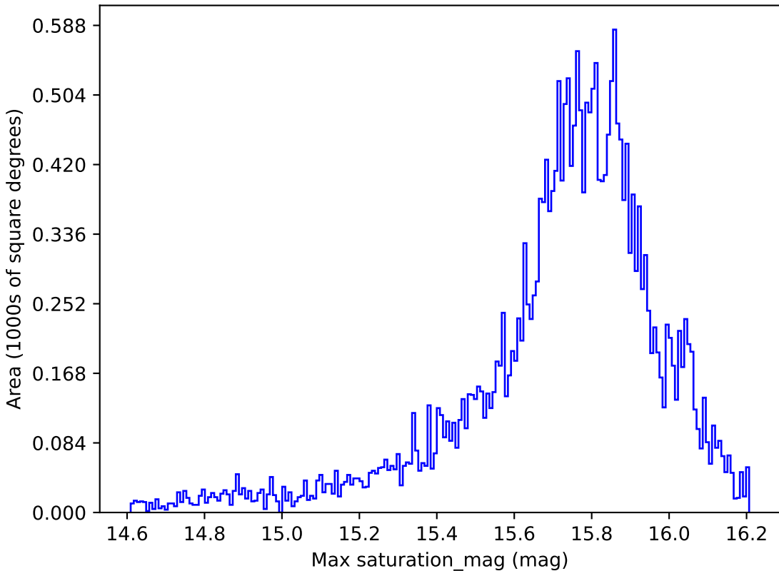
too_ignore_5_4v3.4_10yrs All sky all bands: Max saturation_mag
