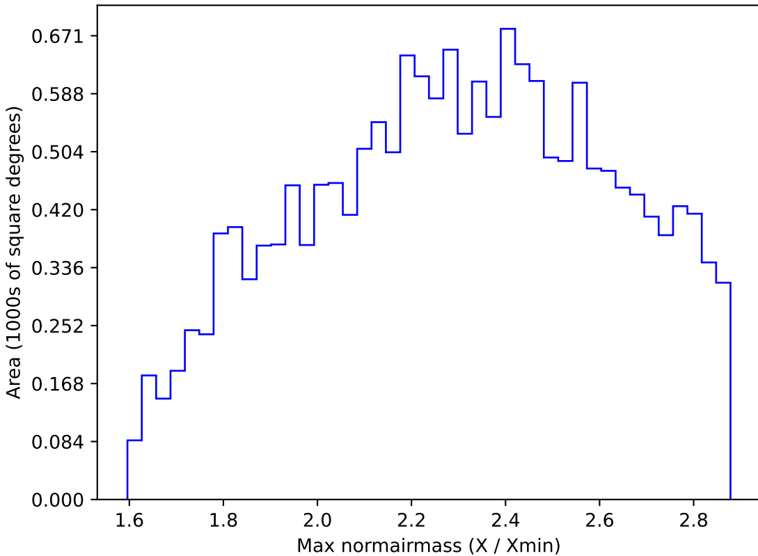
too_ignore_5_4v3.4_10yrs WFD z band: Max normairmass
