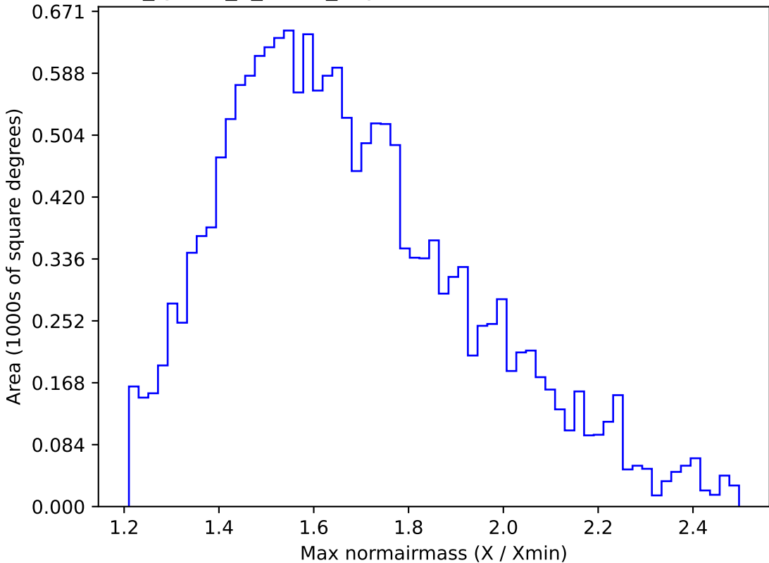
too_ignore_5_4v3.4_10yrs WFD u band: Max normairmass
