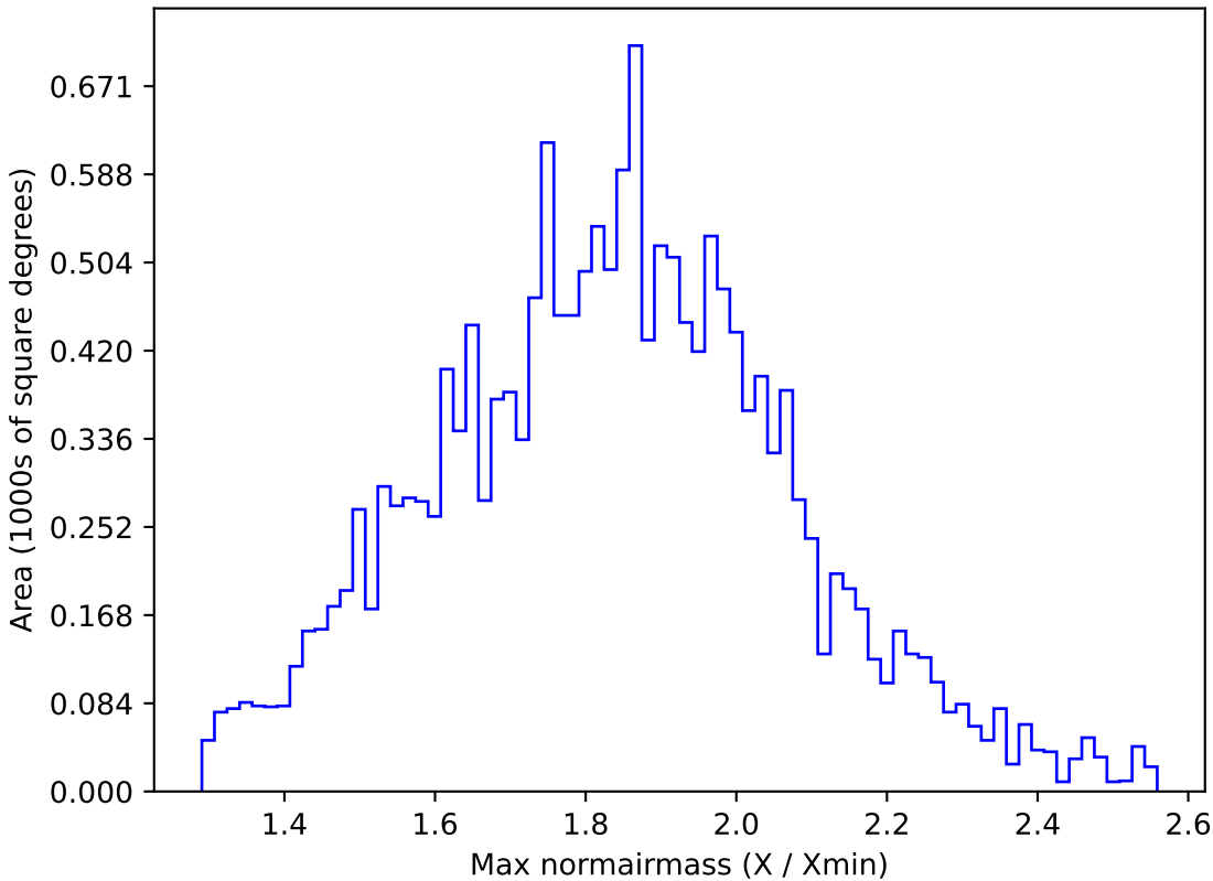
too_ignore_5_4v3.4_10yrs WFD g band: Max normairmass
