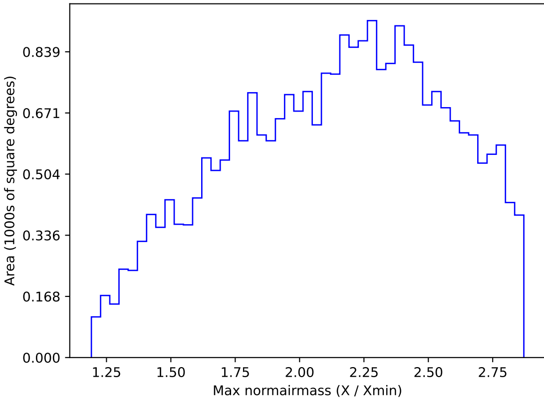
too_ignore_5_4v3.4_10yrs All sky z band: Max normairmass
