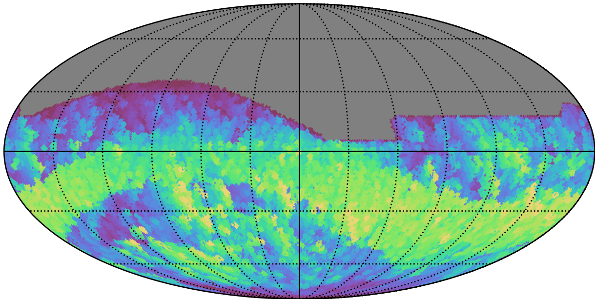
too_ignore_5_4v3.4_10yrs All sky r band: Max normairmass
