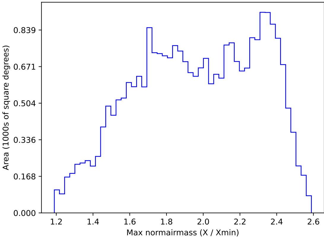
too_ignore_5_4v3.4_10yrs All sky r band: Max normairmass
