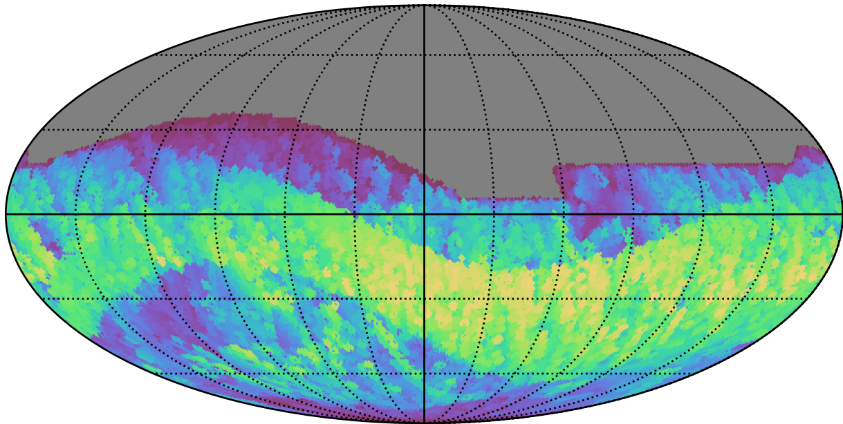
too_ignore_5_4v3.4_10yrs All sky i band: Max normairmass
