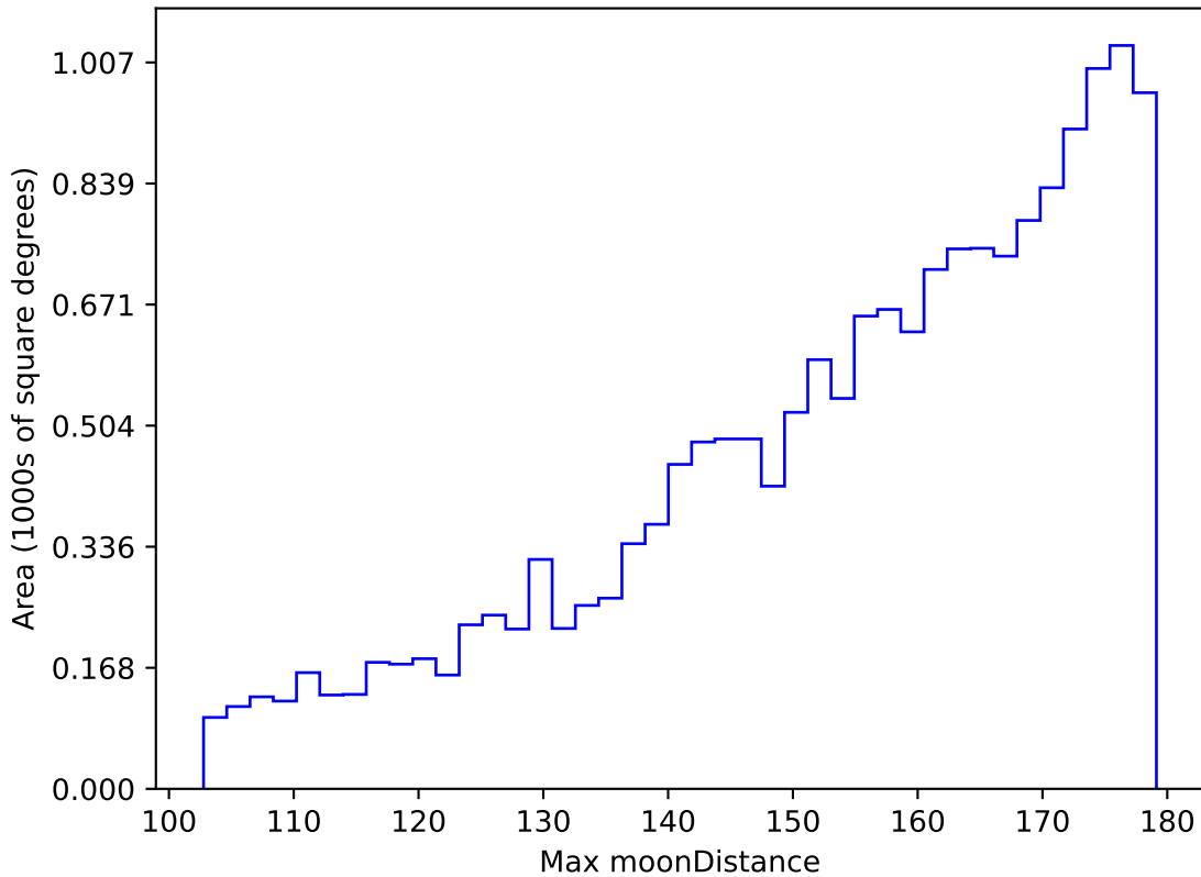
too_ignore_5_4v3.4_10yrs WFD z band: Max moonDistance
