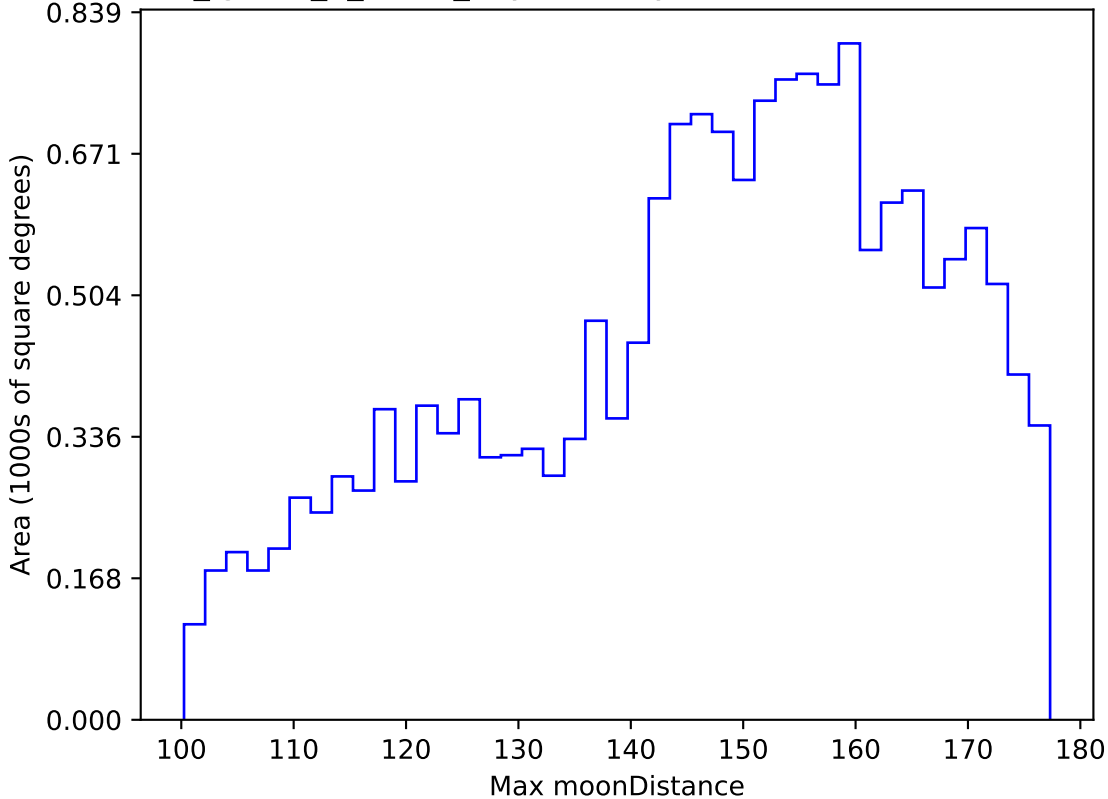
too_ignore_5_4v3.4_10yrs WFD y band: Max moonDistance
